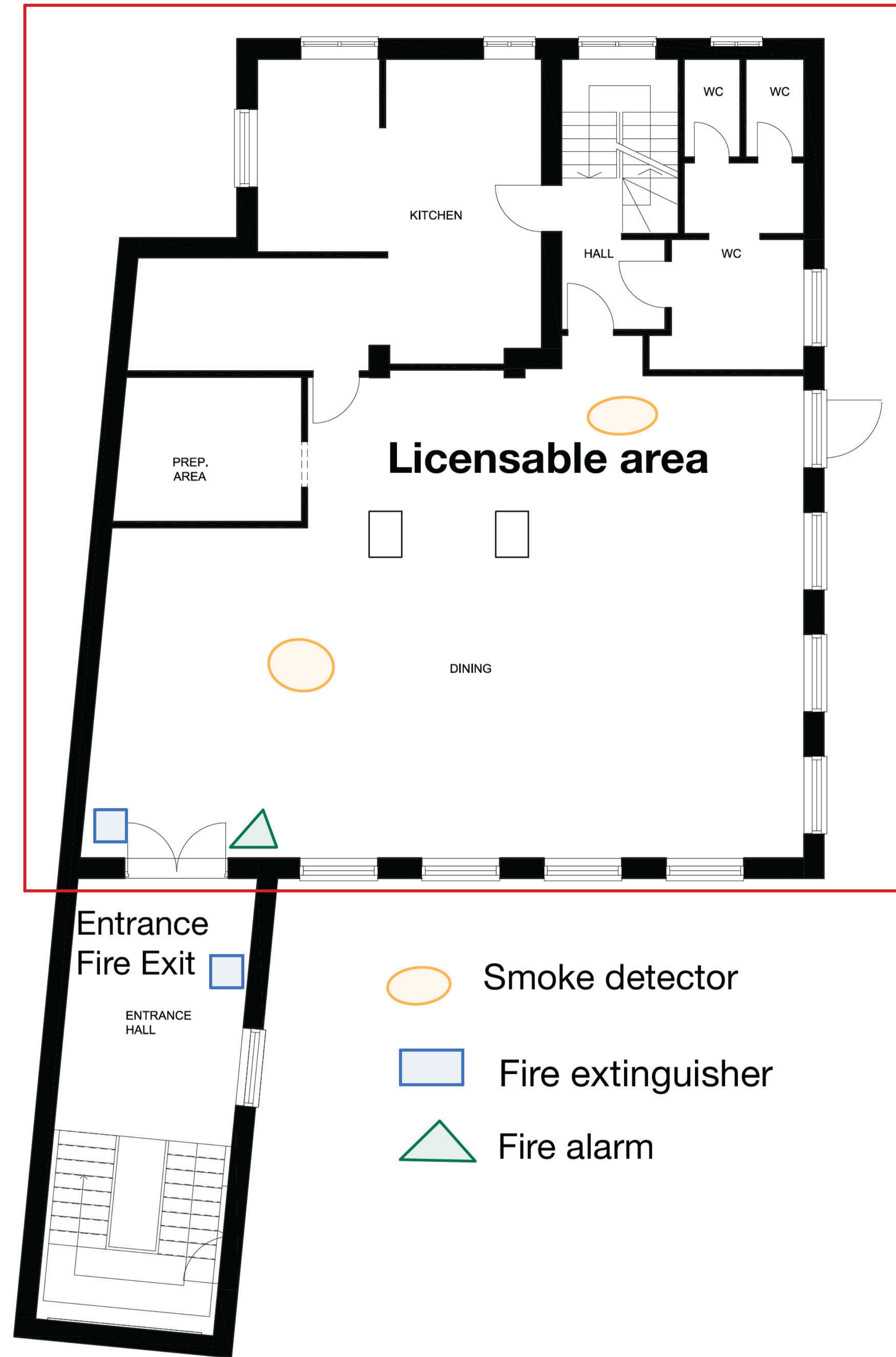
2 EXISTING FIRST FLOOR PLAN 1 : 50
